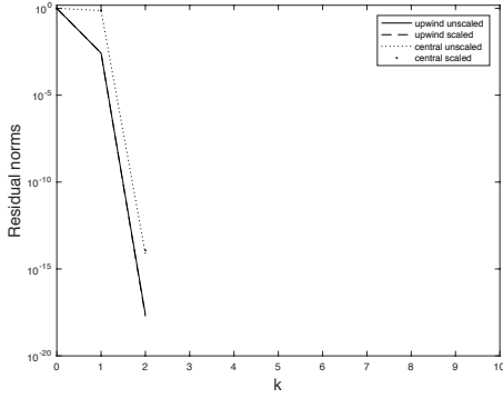
FIG. 5.6. GMRES convergence for \epsilon = 10^{-4} .
