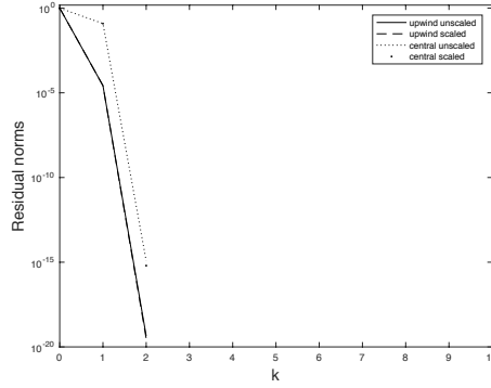
FIG. 5.7. GMRES convergence for \epsilon = 10^{-6} .
