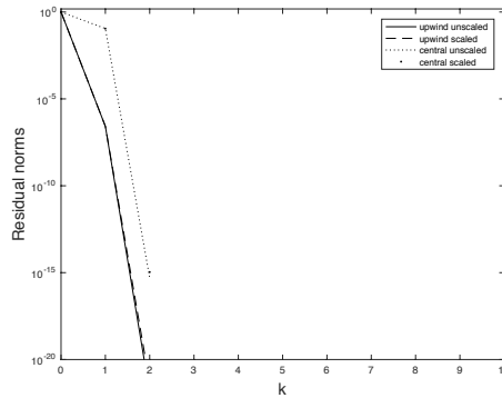
FIG. 5.8. GMRES convergence for \epsilon = 10^{-8} .
