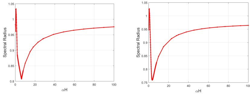
Fig. 1 (a) Spectral Radius of \hat{T}_\delta vs. \bar{\alpha} for \bar{\gamma} = 0.001 , p, q = 10 , k_\delta = 20 and \bar{\alpha} \in [0.1, 100] . (b) Spectral radius of \hat{T}_\delta vs. \bar{\alpha} for p, q = 10 , k_\delta = 20 , \bar{\gamma} = 0.01 and \bar{\alpha} \in [0.1, 100]
