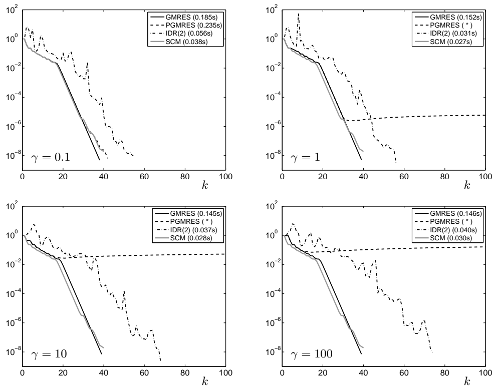
FIG. 5.1. Convergence of the Schur Complement Method for \mathbf{Ax} = \mathbf{b} , with coefficient matrix of dimension n = 10^4 given by the simple example (3.3) with a 2 \times 2 identity added to the \mathbf{Z} block, and parameters \alpha = 0.125 , \beta = 1 , and p = 6 ; the vector \mathbf{b} is equal to 1/\sqrt{n} in all components. The gray line shows the upper bound \gamma_k in (5.1) on the residual norm. For context, the residual norms for full GMRES, PGMRES, and IDR(2) are also shown.
