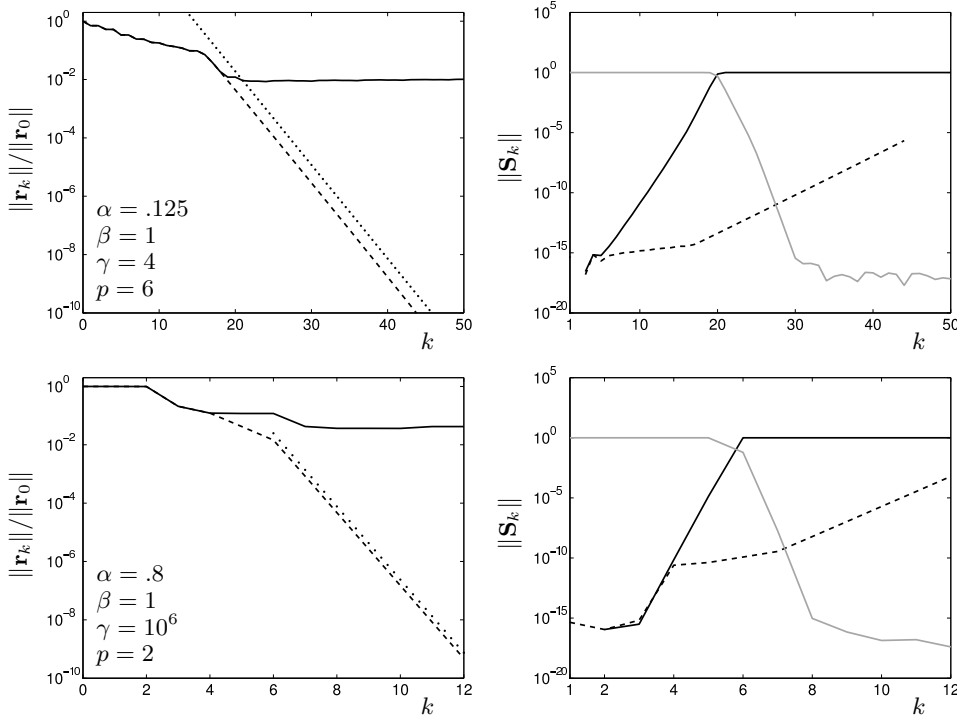
FIG. 3.3. PGMRES (solid line) and standard (modified Gram–Schmidt) GMRES (dashed line) as in Figure 3.1, applied to the simple example (3.3) with a vector \mathbf{b} = [1, \dots, 1]^T and n = 200 . The dotted line in each left plot shows the convergence bound (3.4). The gray line in each right plot shows the smallest singular value of the Arnoldi basis matrix \mathbf{V}_k computed by PGMRES. In the well-conditioned top example ( \text{cond}(\mathbf{A}) = 32 ), the instability develops gradually; in the ill-conditioned bottom example ( \text{cond}(\mathbf{A}) = 1.25 \times 10^6 ), the instability is apparent at the fifth iteration.
